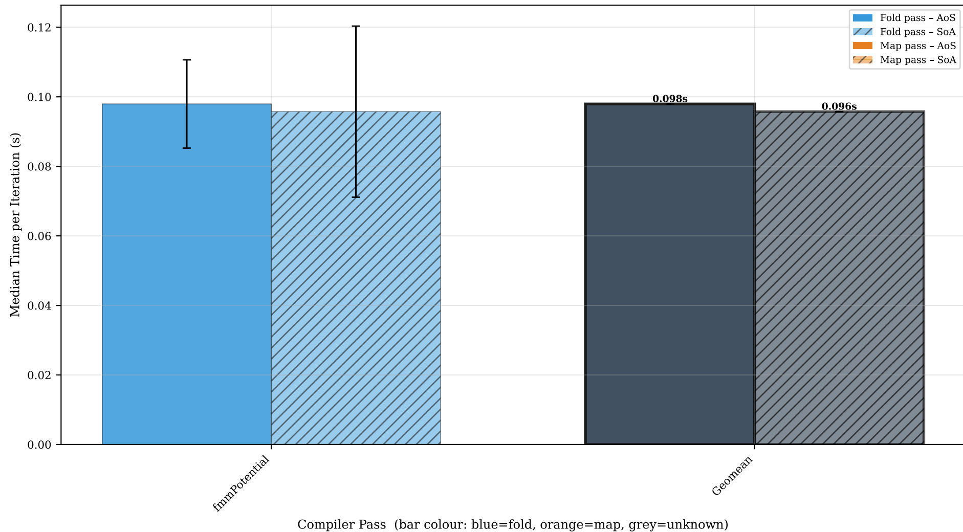
OctTree fmmPotential — AoS (solid) vs SoA (hatched), all passes (error bars = std dev, rightmost bar = geomean)
