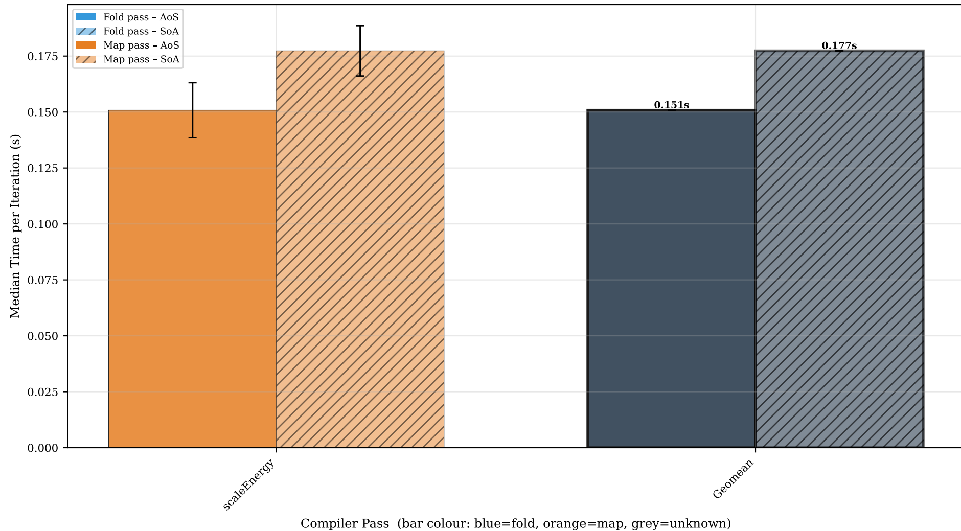
OctTree_scaleEnergy — AoS (solid) vs SoA (hatched), all passes (error bars = std dev, rightmost bar = geomean)
