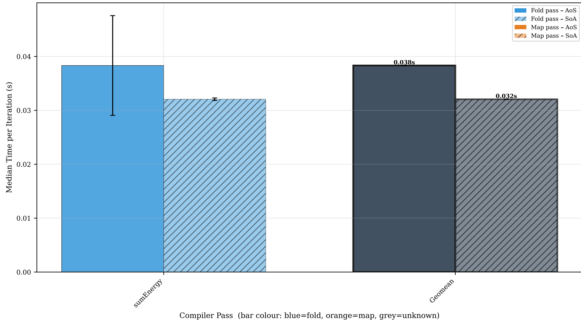
OctTree_sumEnergy — AoS (solid) vs SoA (hatched), all passes (error bars = std dev, rightmost bar = geomean)
