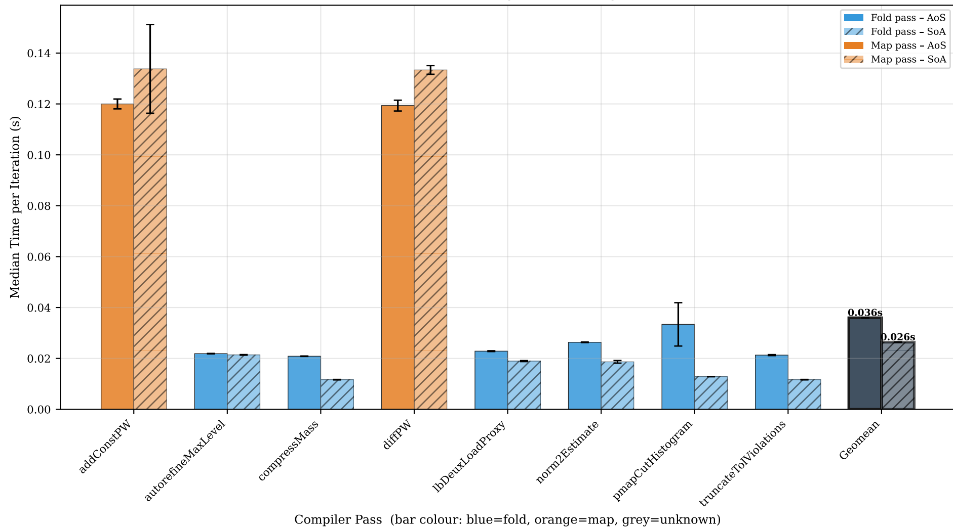
PiecewiseFunctions — AoS (solid) vs SoA (hatched), all passes (error bars = std dev, rightmost bar = geomean)
