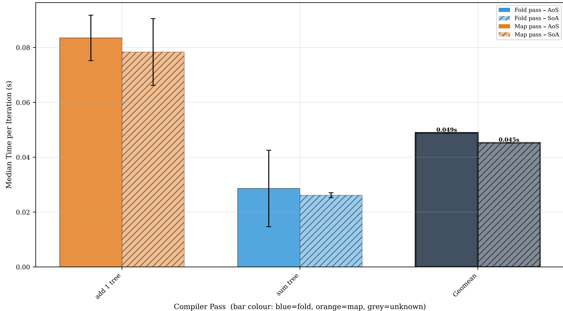
TernaryTree — AoS (solid) vs SoA (hatched), all passes (error bars = std dev, rightmost bar = geomean)
