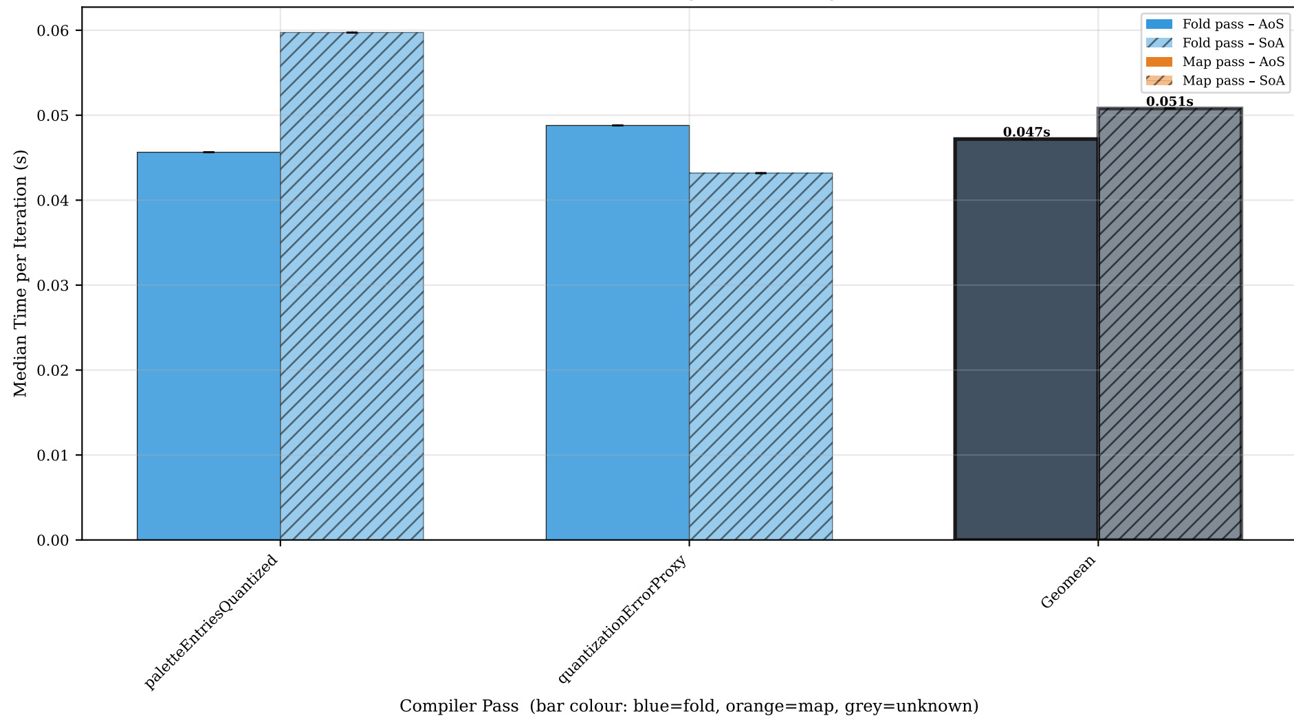
ColorOctree — AoS (solid) vs SoA (hatched), all passes (error bars = std dev, rightmost bar = geomean)
