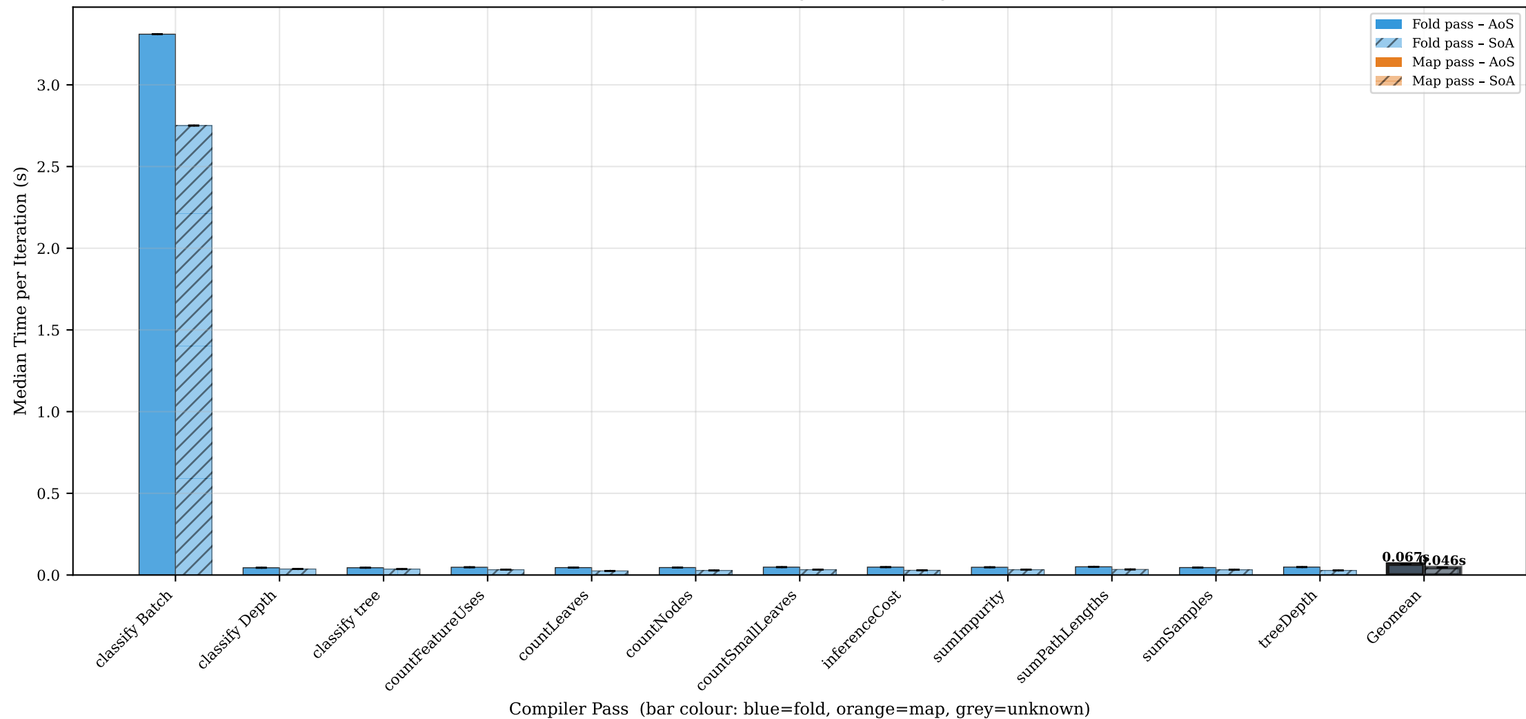
DecisionTree — AoS (solid) vs SoA (hatched), all passes (error bars = std dev, rightmost bar = geomean)
