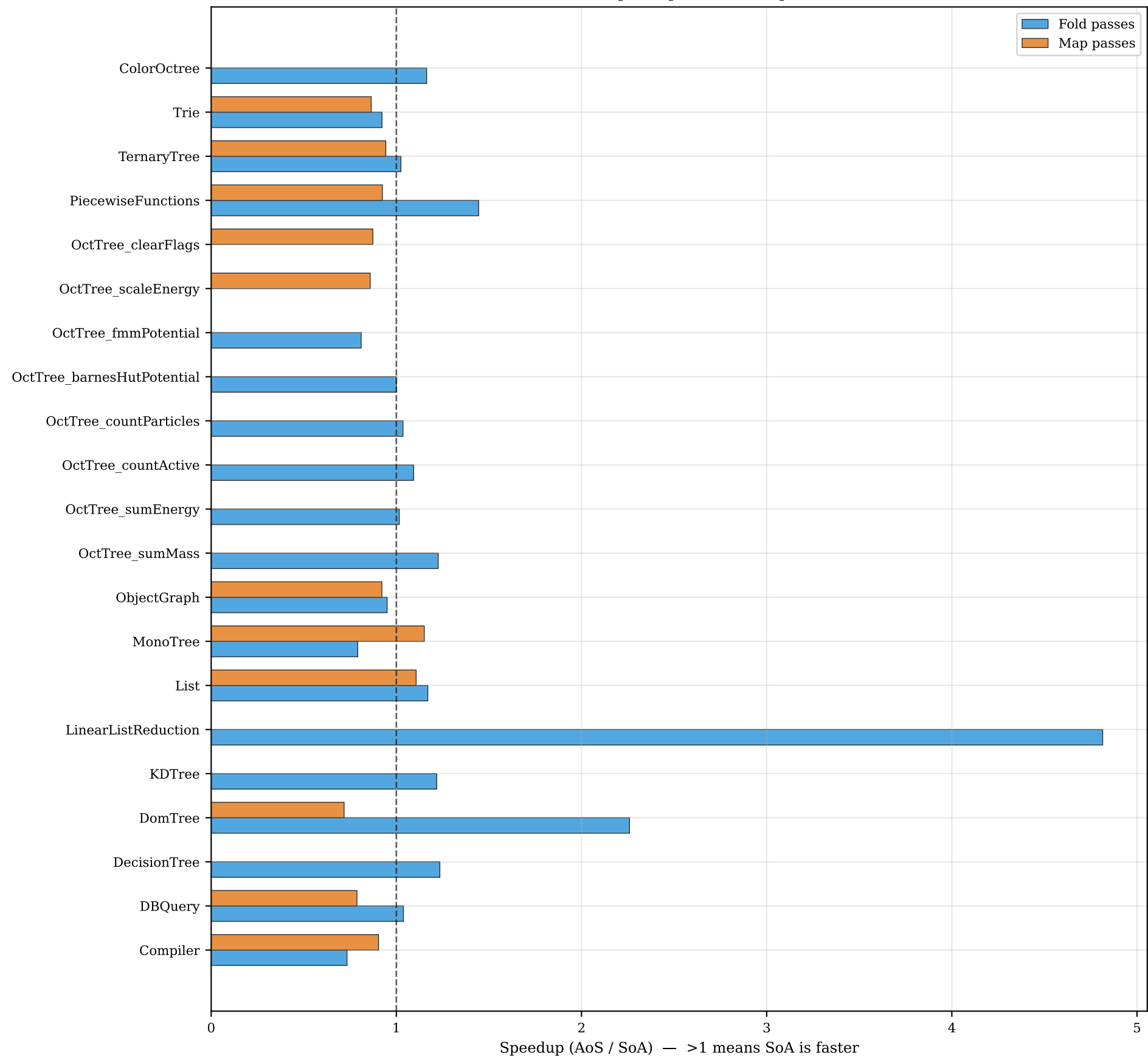
End-to-End Speedup: Fold vs Map Passes
