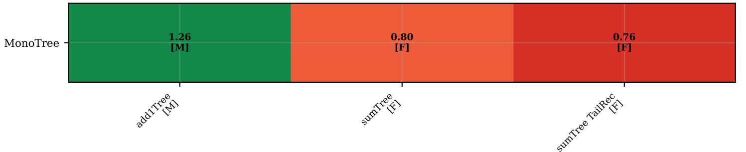
MonoTree: per-pass speedup heatmap (F=fold M=map ?=unknown | SoA=2 buffers total)
