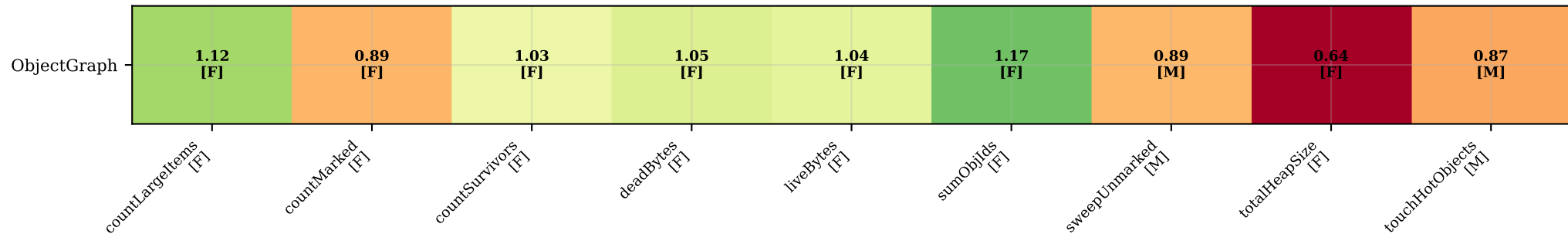
ObjectGraph: per-pass speedup heatmap (F=fold M=map ?=unknown | SoA=4 buffers total)
