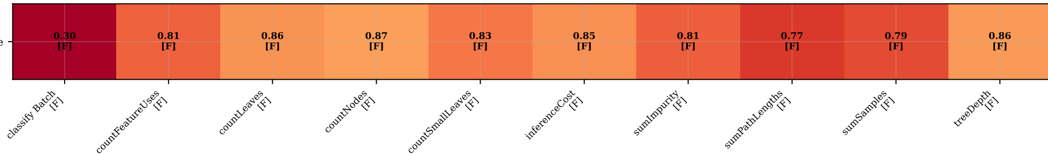
DecisionTree: per-pass speedup heatmap (F=fold M=map ?=unknown | SoA=6 buffers total)
