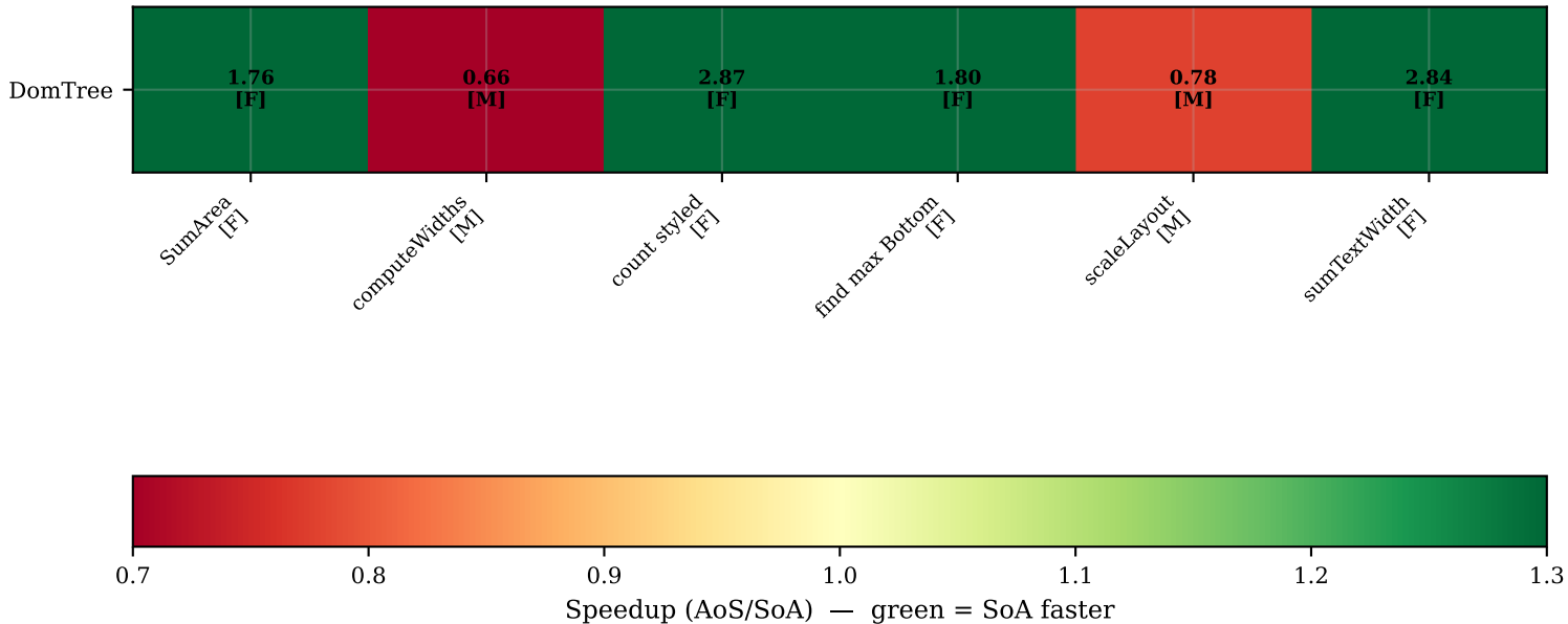
DomTree: per-pass speedup heatmap (F=fold M=map ?=unknown | SoA=14 buffers total)
