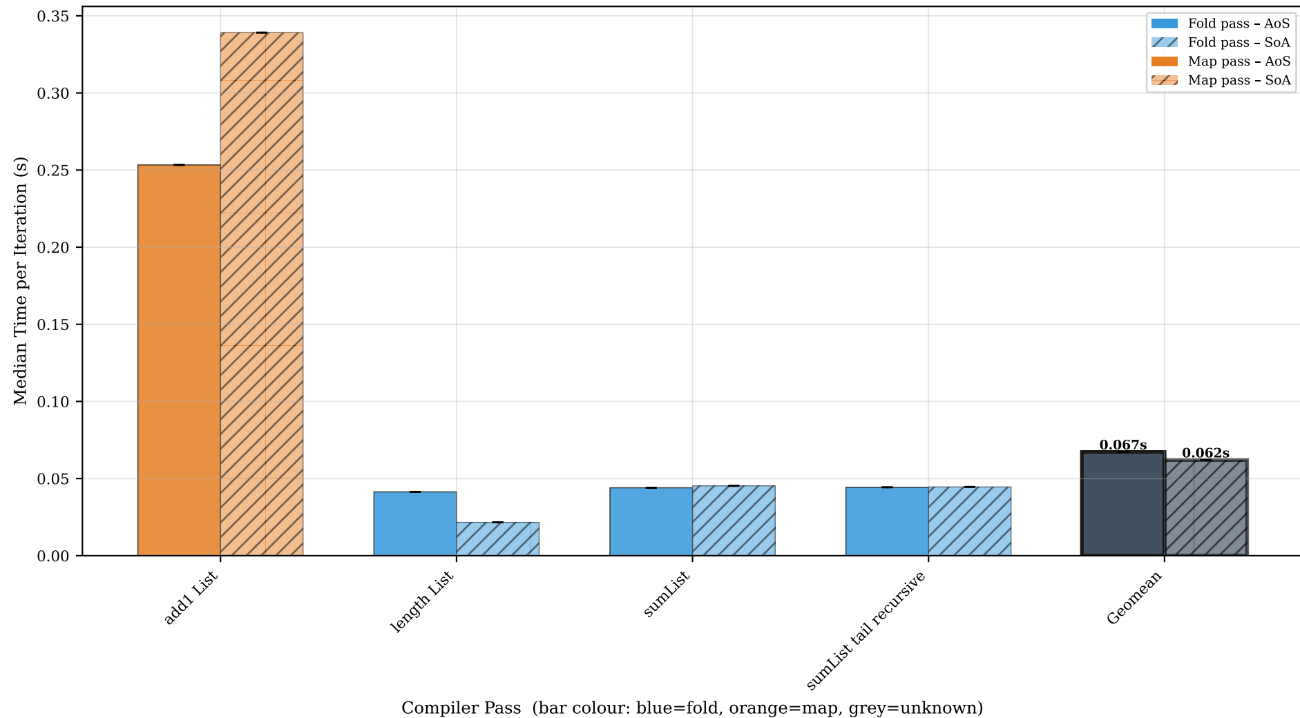
List — AoS (solid) vs SoA (hatched), all passes (error bars = std dev, rightmost bar = geomean)
