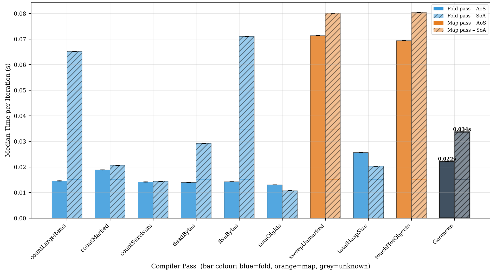
ObjectGraph — AoS (solid) vs SoA (hatched), all passes (error bars = std dev, rightmost bar = geomean)
