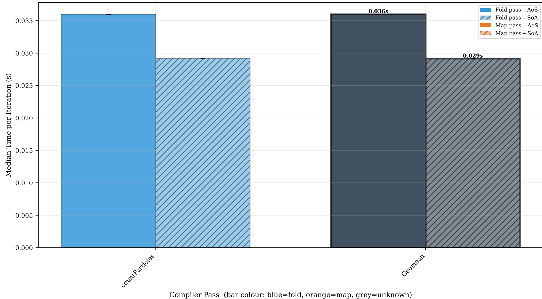
OctTree_countParticles — AoS (solid) vs SoA (hatched), all passes (error bars = std dev, rightmost bar = geomean)
