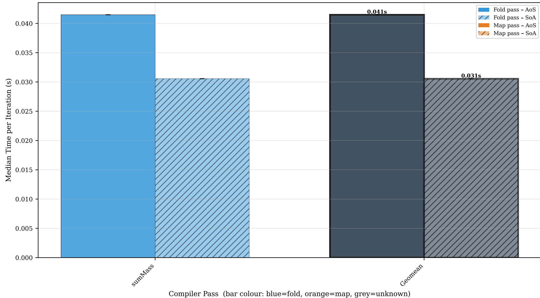
OctTree_sumMass — AoS (solid) vs SoA (hatched), all passes (error bars = std dev, rightmost bar = geomean)
