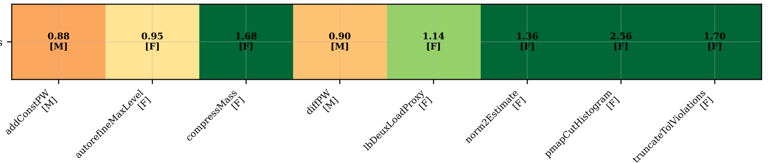
PiecewiseFunctions: per-pass speedup heatmap (F=fold M=map ?=unknown | SoA=7 buffers total)
