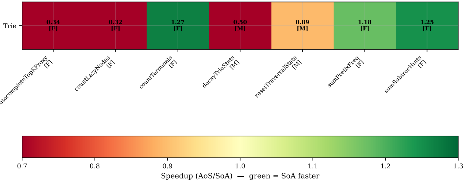
Trie: per-pass speedup heatmap (F=fold M=map ?=unknown | SoA=9 buffers total)
