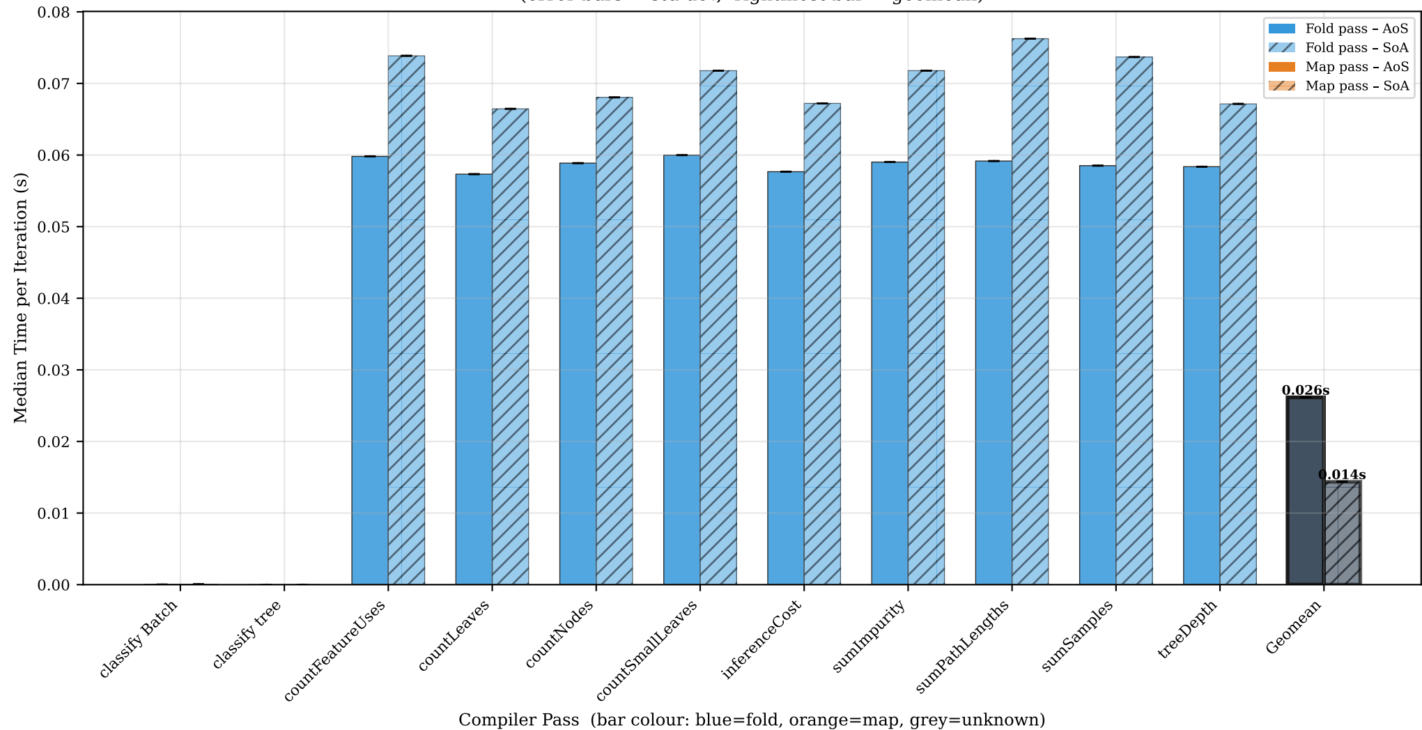
DecisionTree — AoS (solid) vs SoA (hatched), all passes (error bars = std dev, rightmost bar = geomean)
