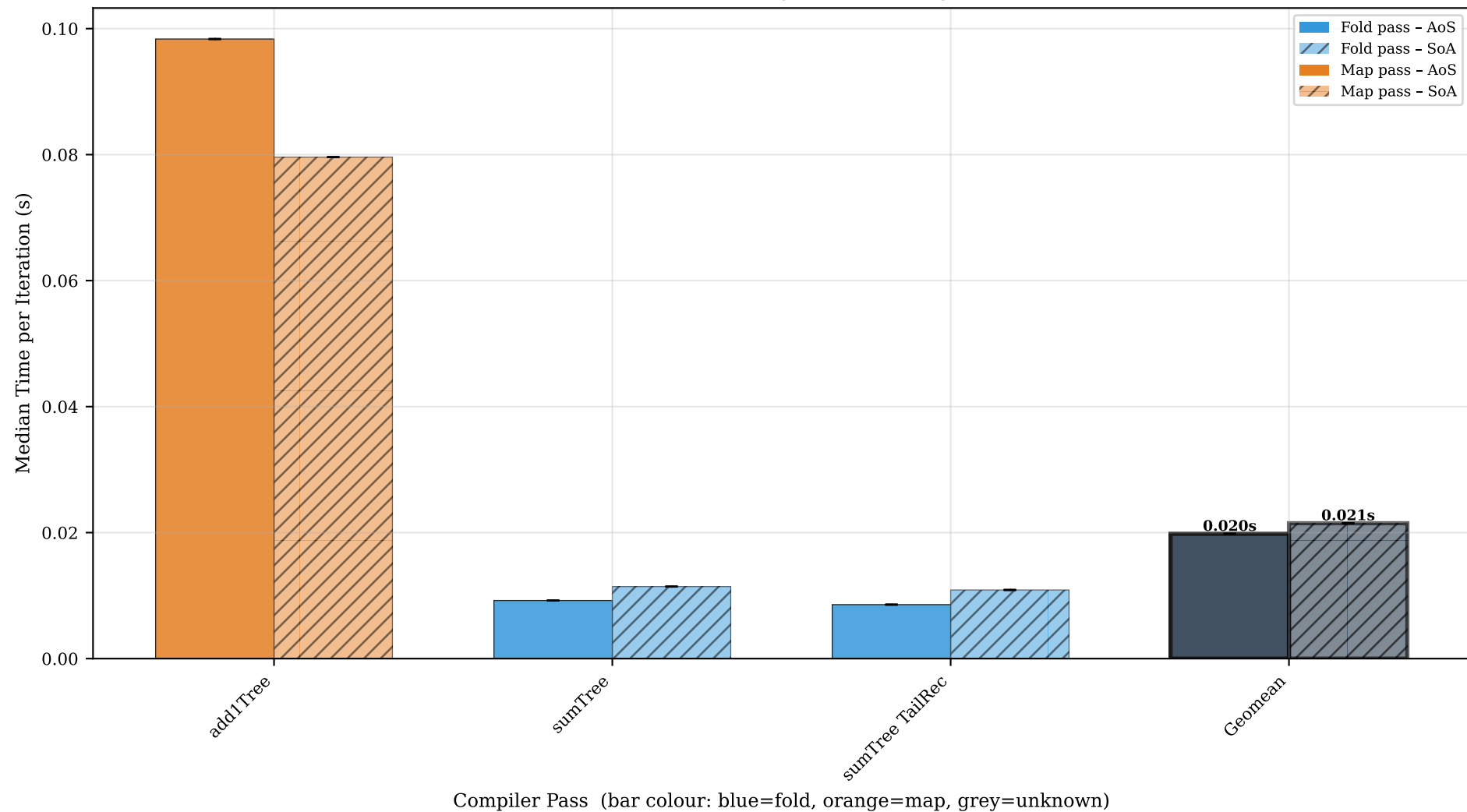
MonoTree — AoS (solid) vs SoA (hatched), all passes (error bars = std dev, rightmost bar = geomean)
