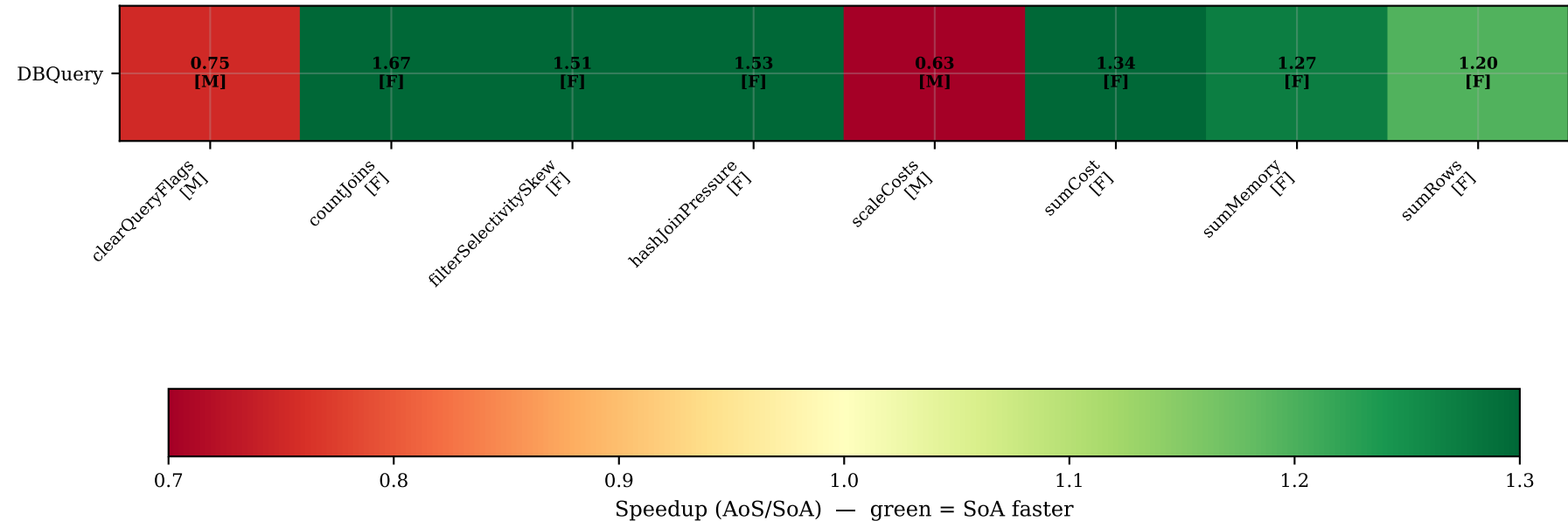
DBQuery: per-pass speedup heatmap (F=fold M=map ?=unknown | SoA=13 buffers total)
