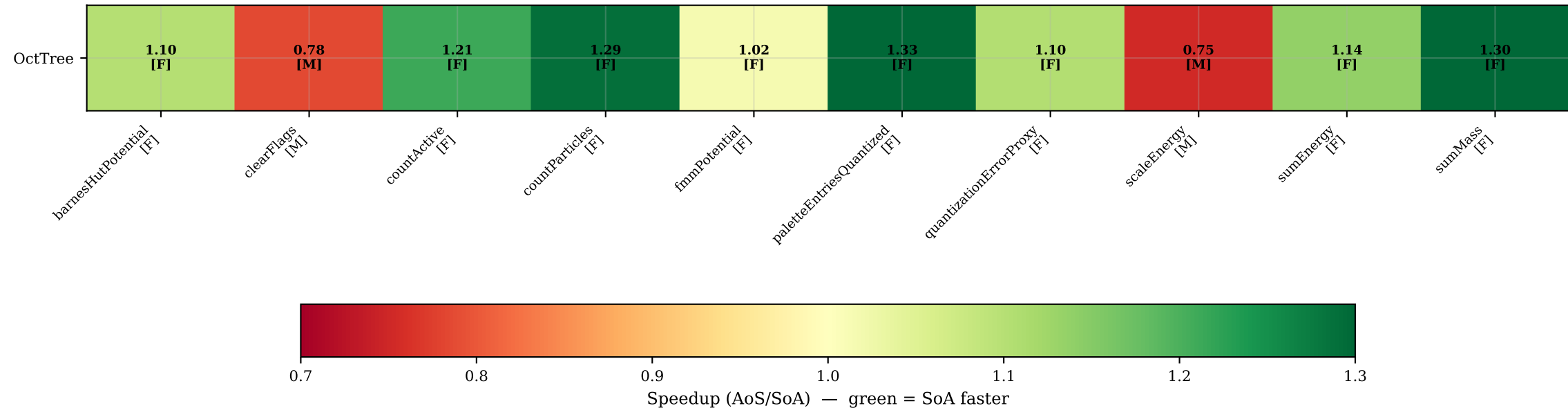
OctTree: per-pass speedup heatmap (F=fold M=map ?=unknown | SoA=18 buffers total)
