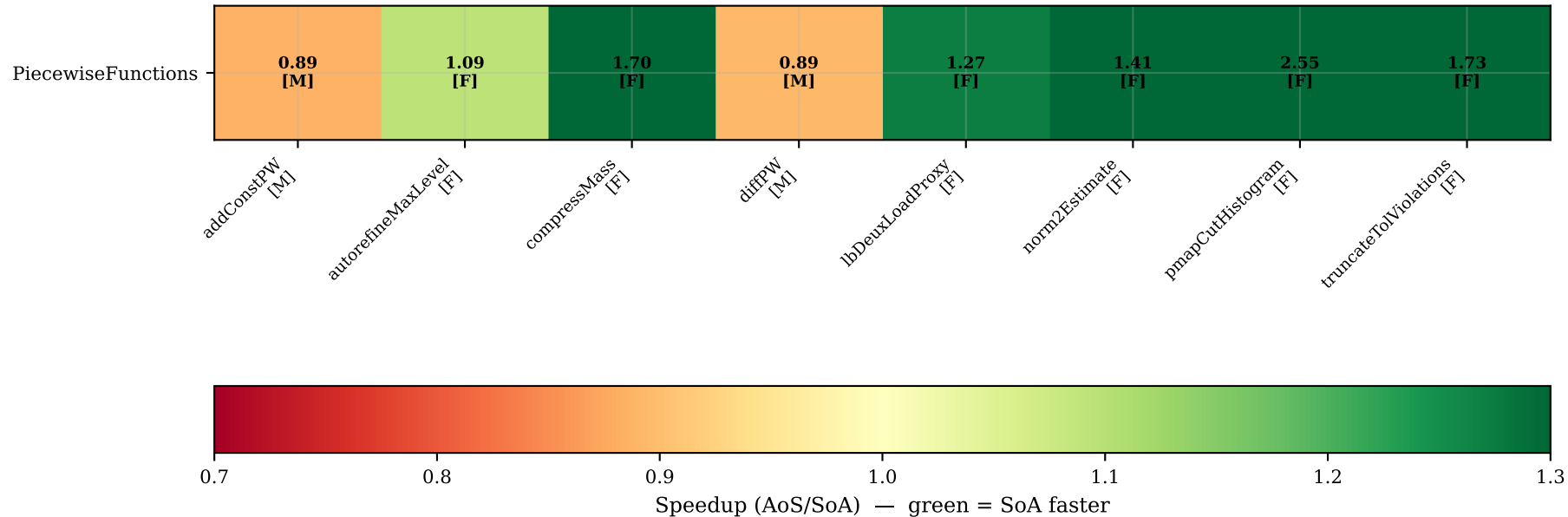
PiecewiseFunctions: per-pass speedup heatmap (F=fold M=map ?=unknown | SoA=7 buffers total)
