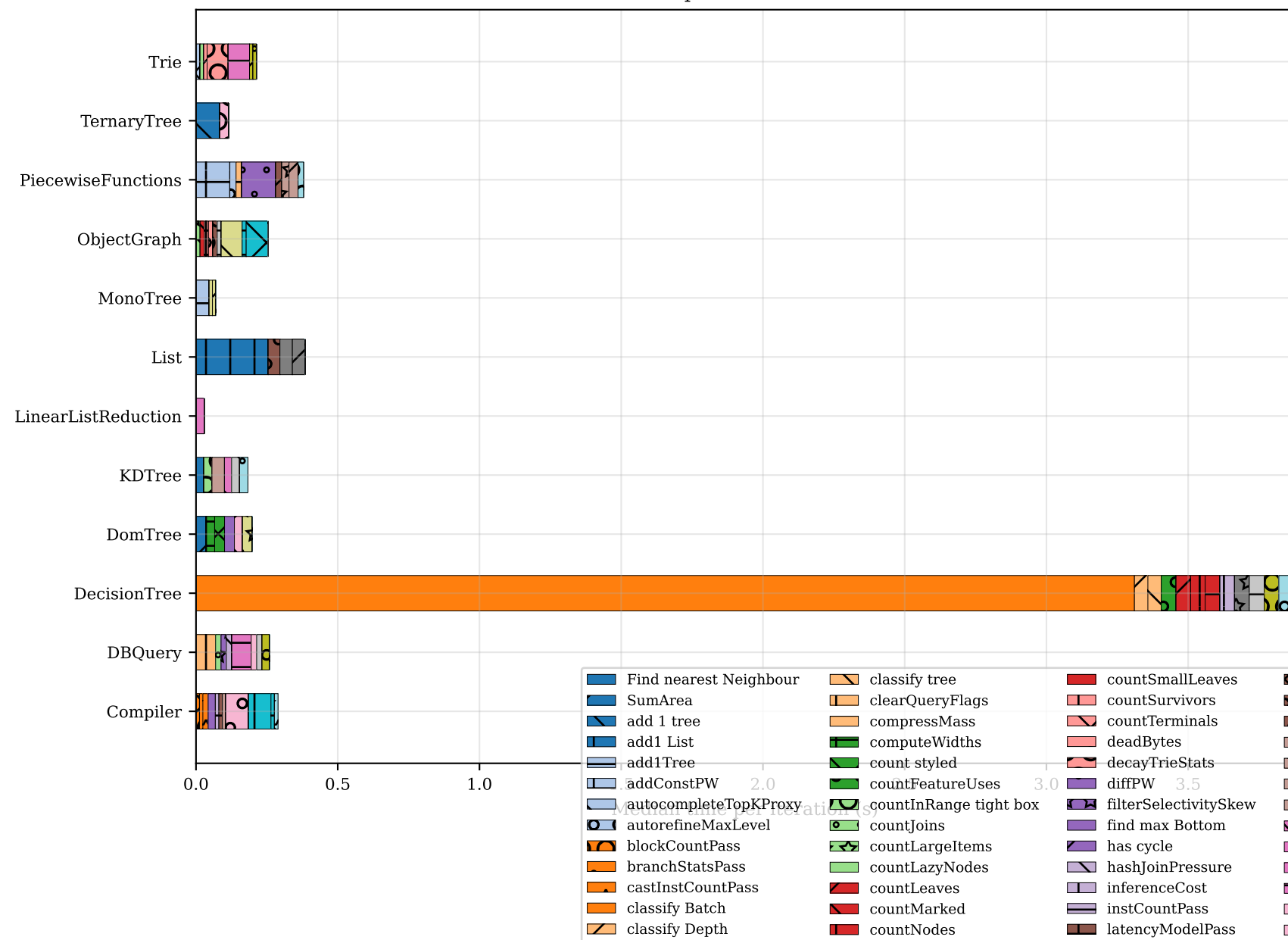
AOS: Complete Pass Breakdown
