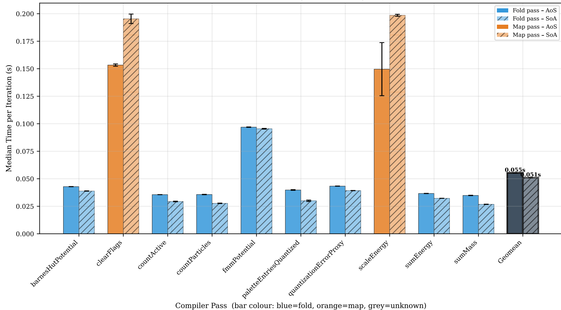
OctTree — AoS (solid) vs SoA (hatched), all passes (error bars = std dev, rightmost bar = geomean)
