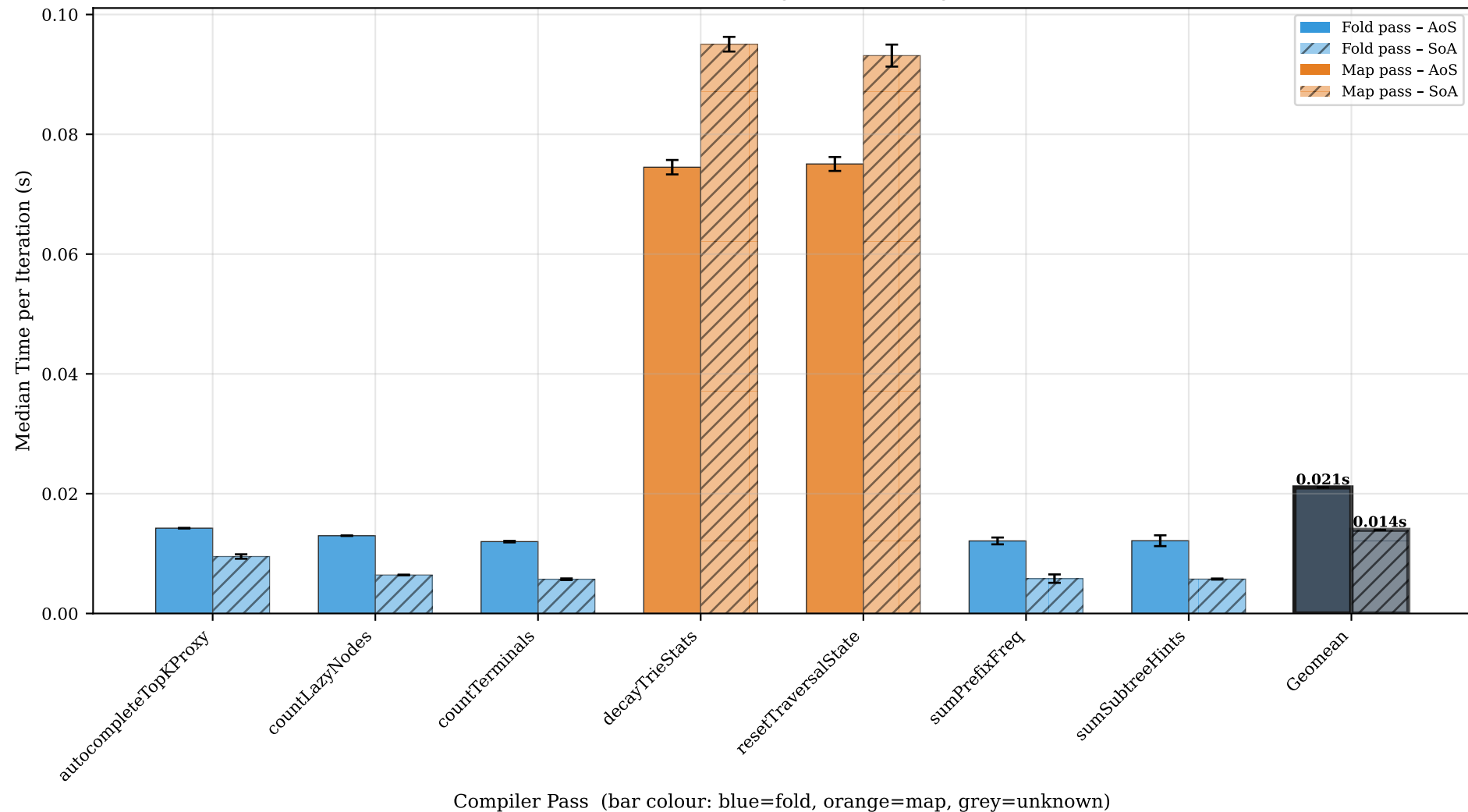
Trie — AoS (solid) vs SoA (hatched), all passes (error bars = std dev, rightmost bar = geomean)
