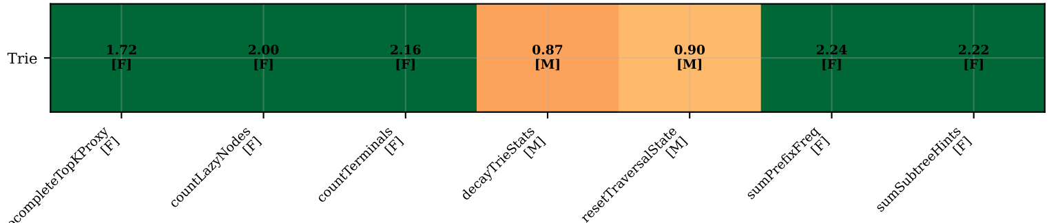
Trie: per-pass speedup heatmap (F=fold M=map ?=unknown | SoA=9 buffers total)
