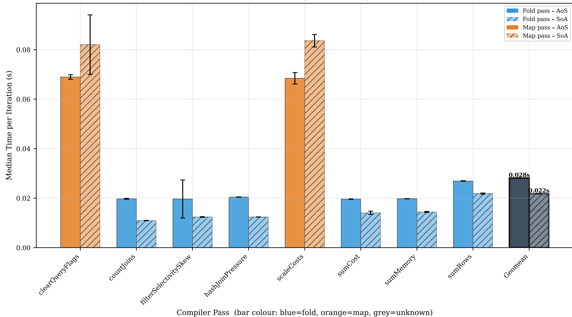
DBQuery — AoS (solid) vs SoA (hatched), all passes (error bars = std dev, rightmost bar = geomean)
