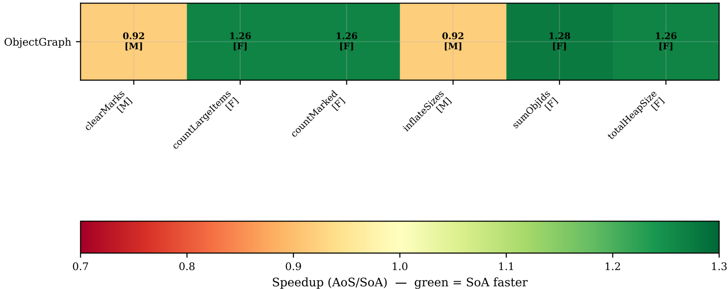
ObjectGraph: per-pass speedup heatmap (F=fold M=map ?=unknown | SoA=4 buffers total)
