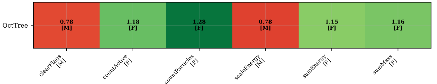
OctTree: per-pass speedup heatmap (F=fold M=map ?=unknown | SoA=9 buffers total)
