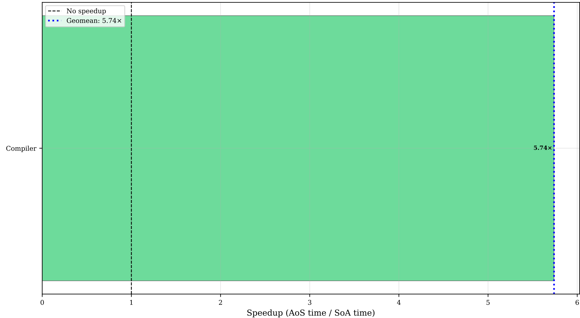
blockCount (fold): Speedup Across All Programs (>1.0 means SoA is faster)
