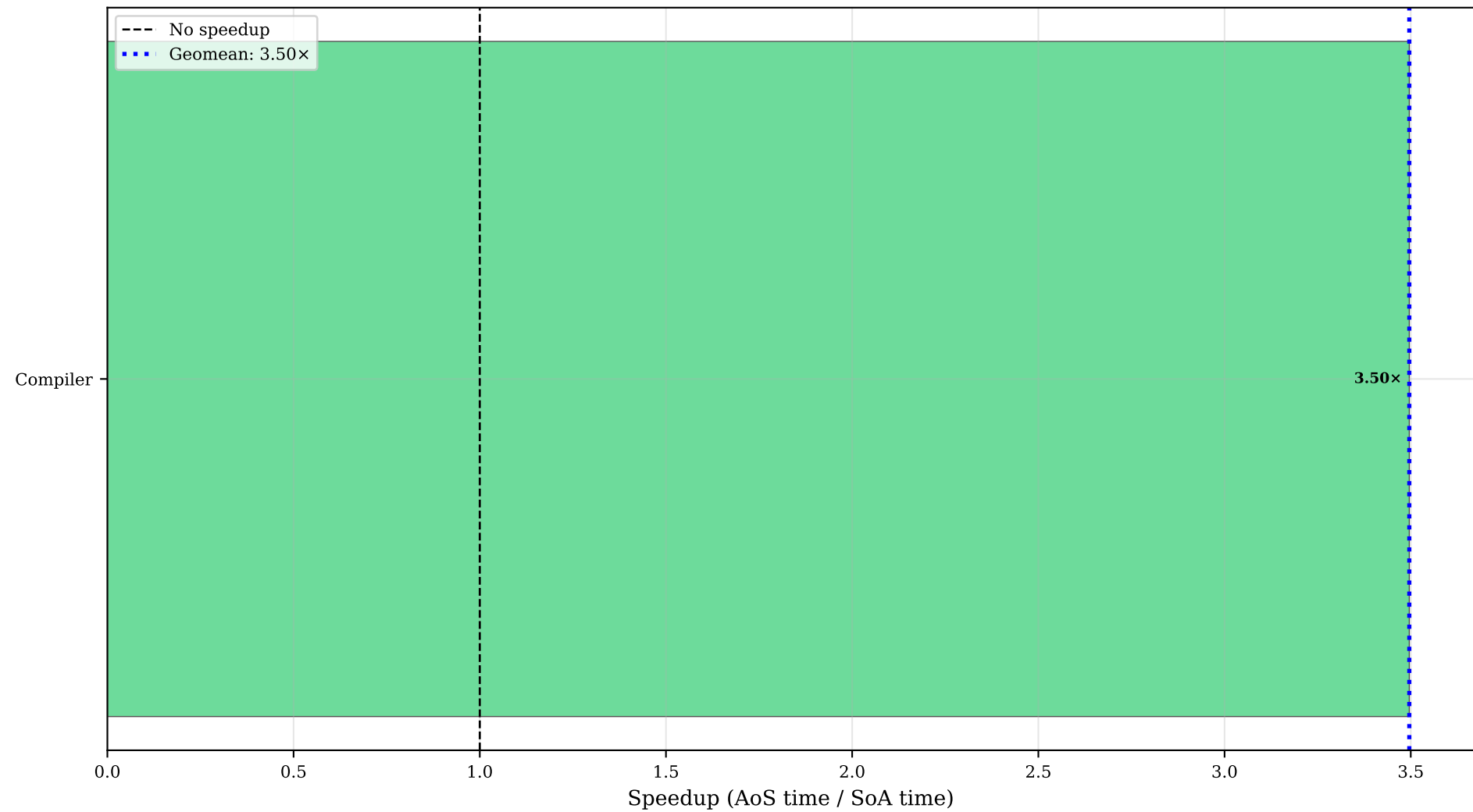
branchStats (fold): Speedup Across All Programs (>1.0 means SoA is faster)
