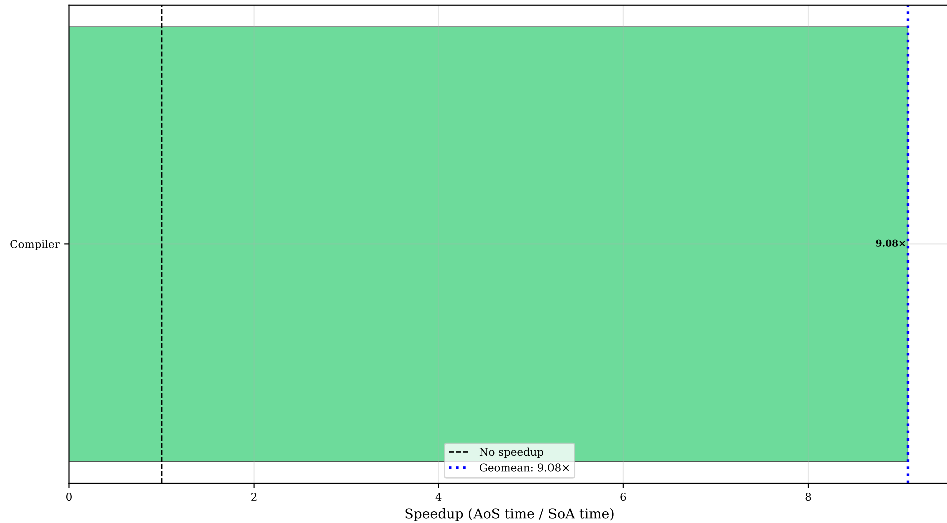
castInstCount (fold): Speedup Across All Programs (>1.0 means SoA is faster)
