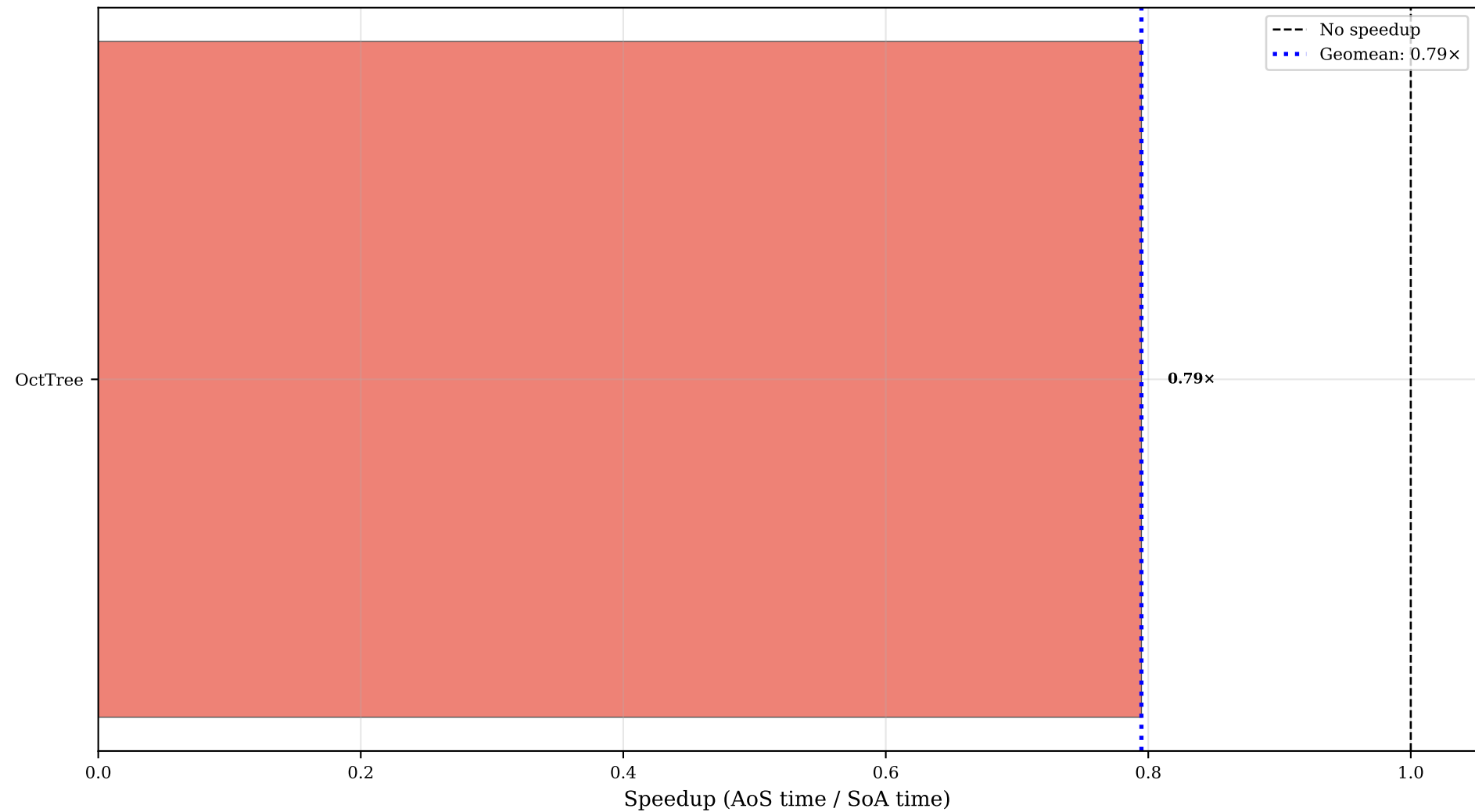
clearFlags (map): Speedup Across All Programs ( >1.0 means SoA is faster)
