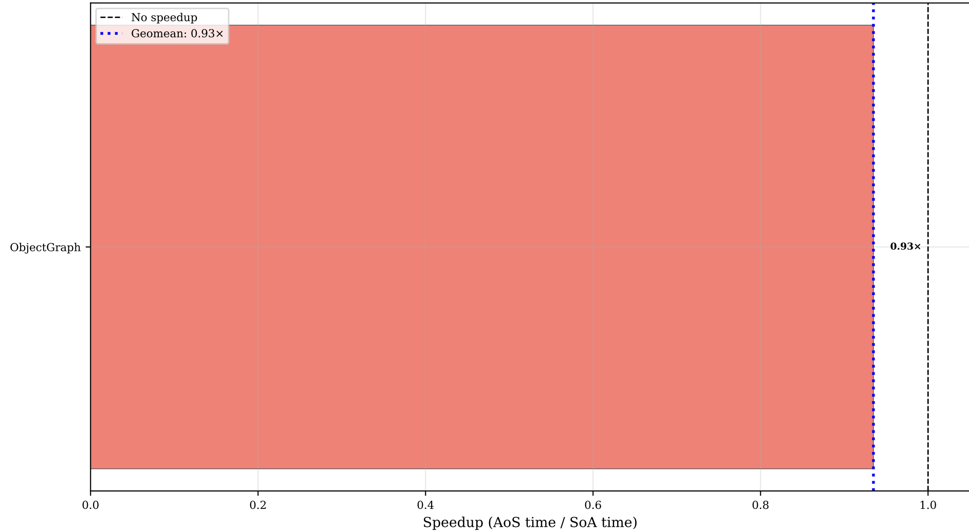
clearMarks (map): Speedup Across All Programs ( >1.0 means SoA is faster)
