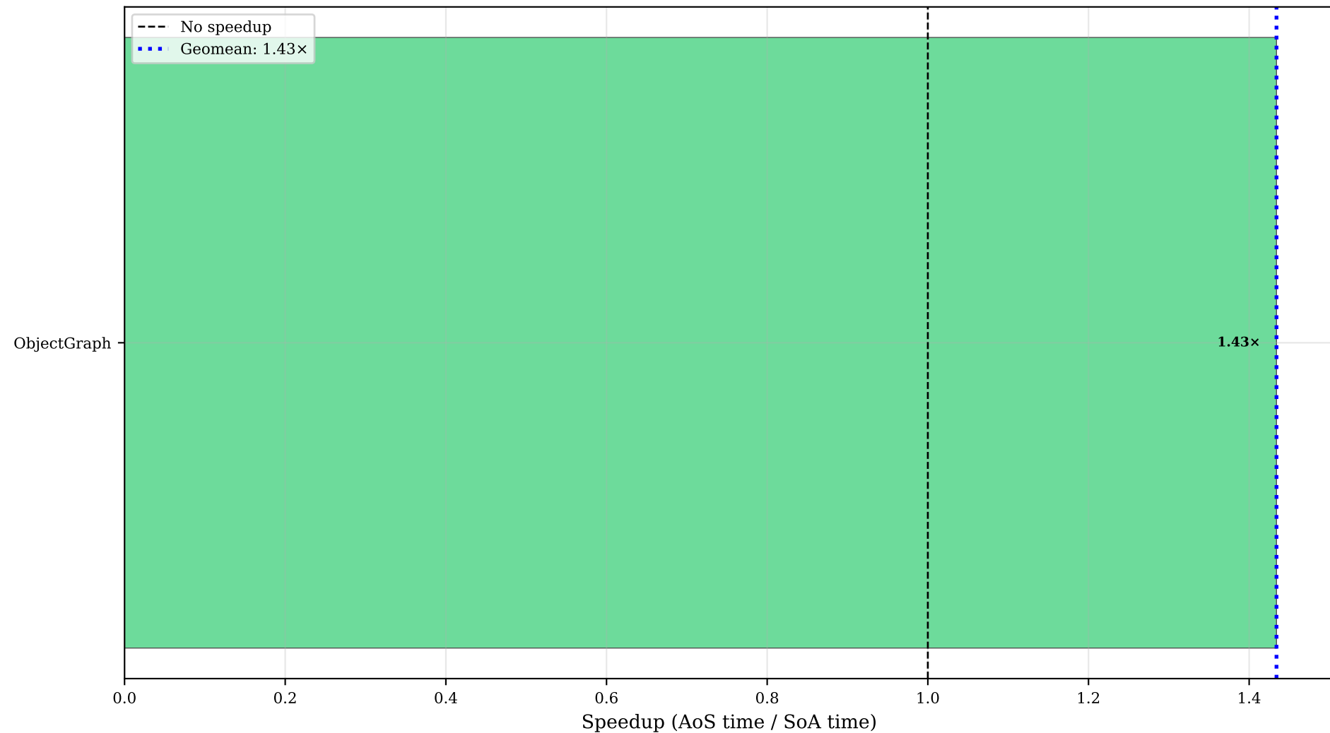
countLargeItems (fold): Speedup Across All Programs (>1.0 means SoA is faster)
