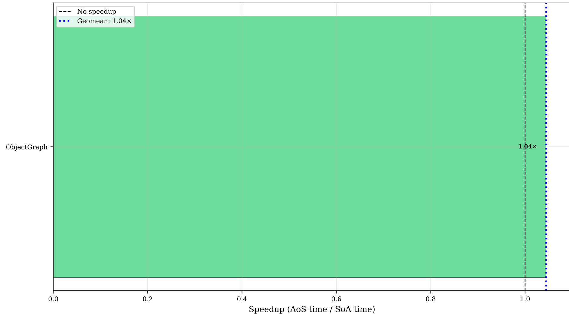
countMarked (fold): Speedup Across All Programs ( >1.0 means SoA is faster)
