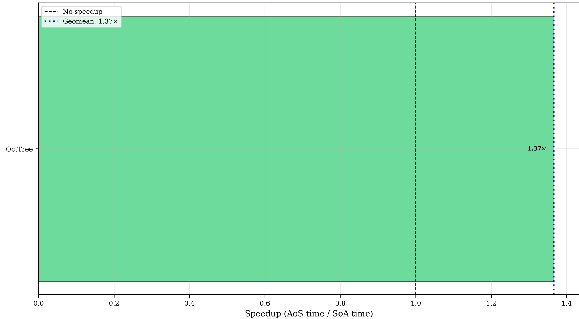
countParticles (fold): Speedup Across All Programs ( >1.0 means SoA is faster)
