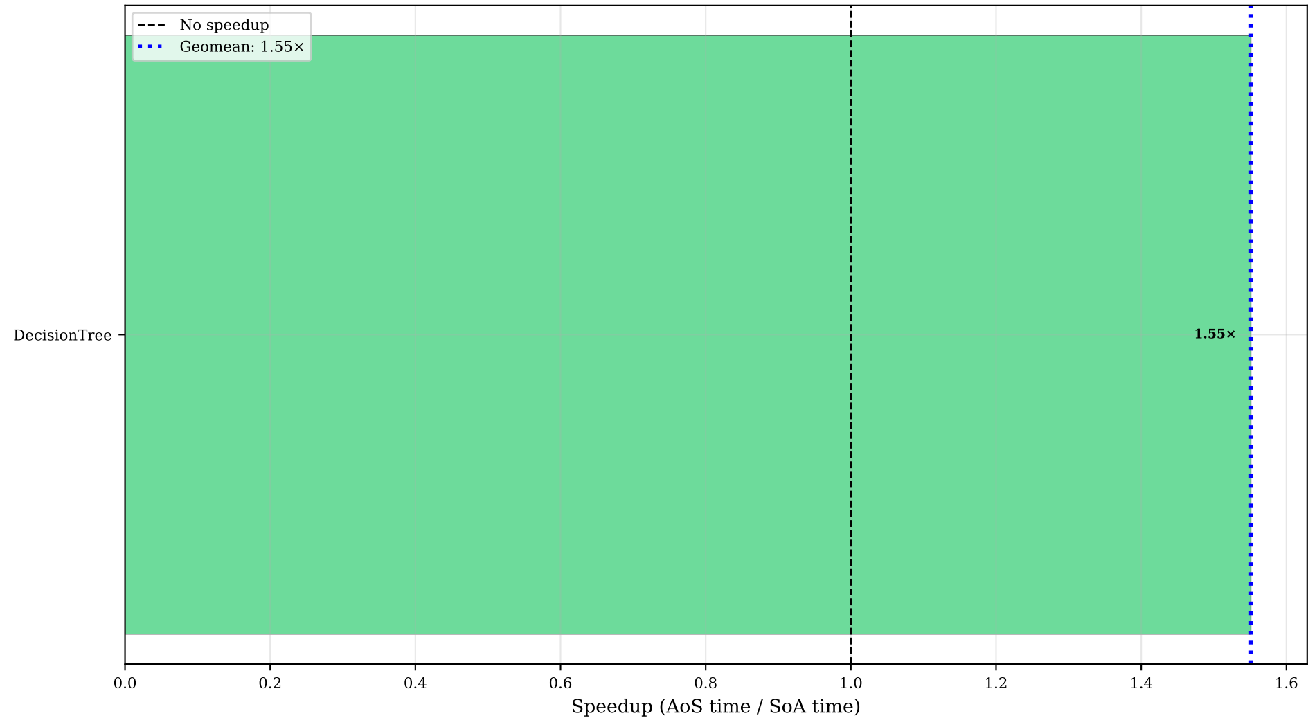
countSmallLeaves (fold): Speedup Across All Programs ( >1.0 means SoA is faster)
