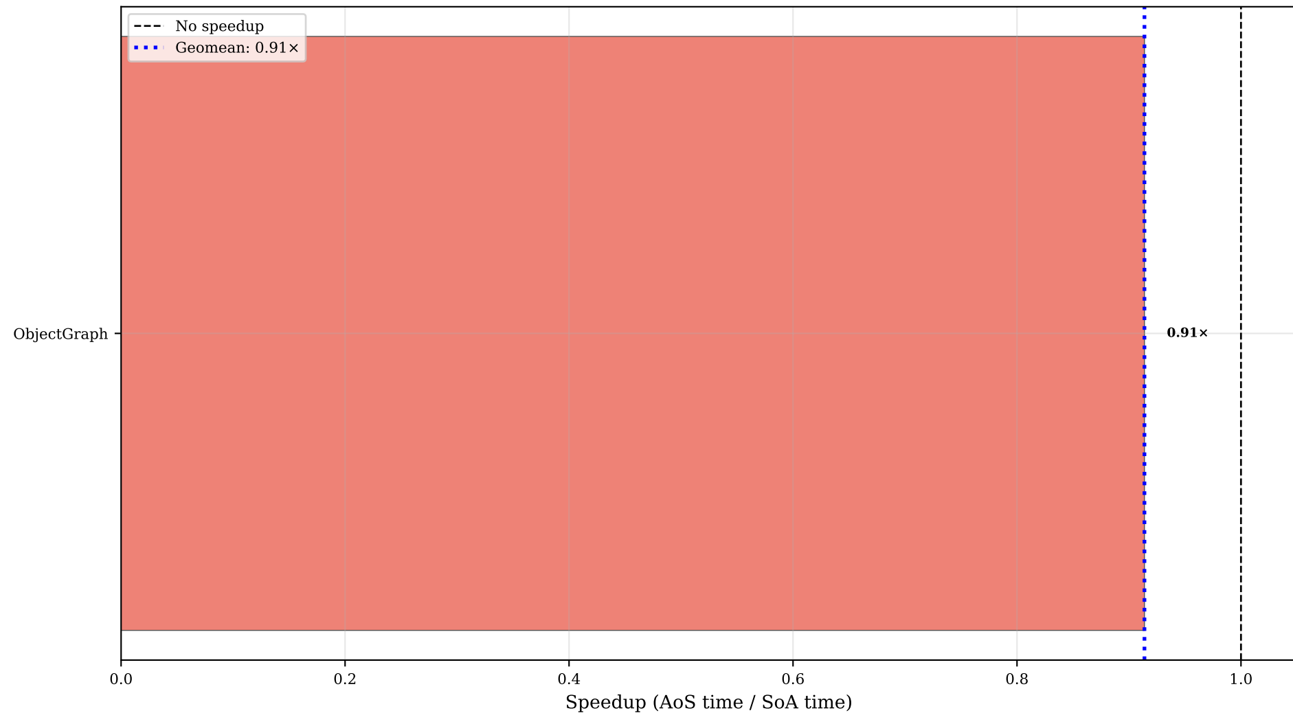
inflateSizes (map): Speedup Across All Programs ( >1.0 means SoA is faster)
