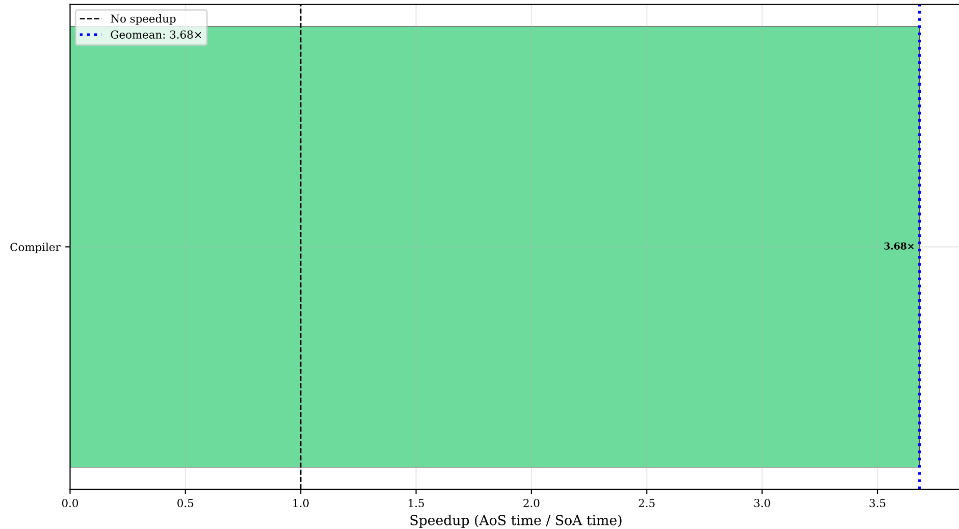
latencyModel (fold): Speedup Across All Programs ( >1.0 means SoA is faster)
