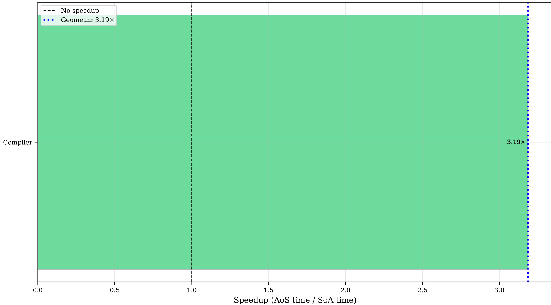
memoryOpStats (fold): Speedup Across All Programs (>1.0 means SoA is faster)
