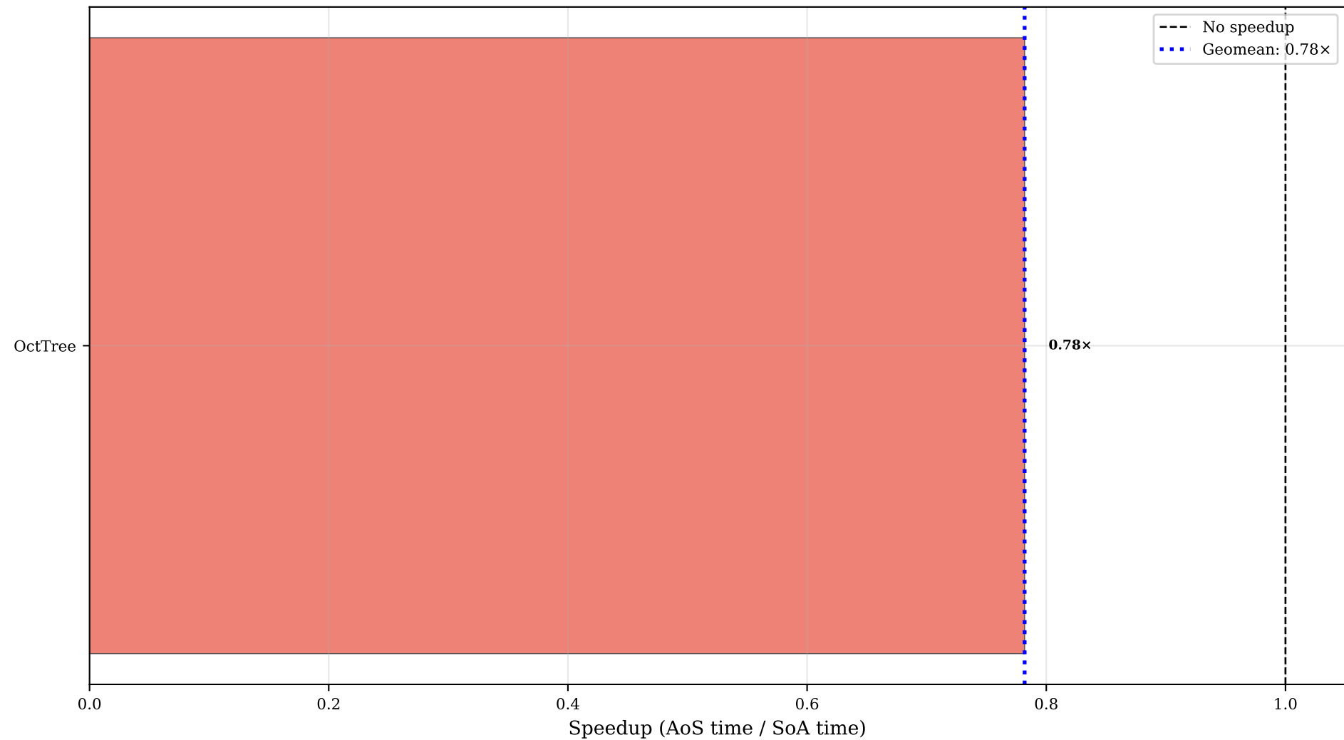
scaleEnergy (map): Speedup Across All Programs ( >1.0 means SoA is faster)
