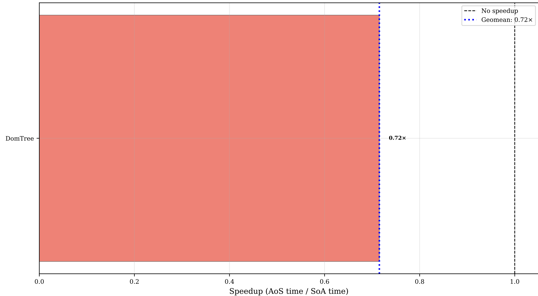
scaleLayout (map): Speedup Across All Programs ( >1.0 means SoA is faster)
