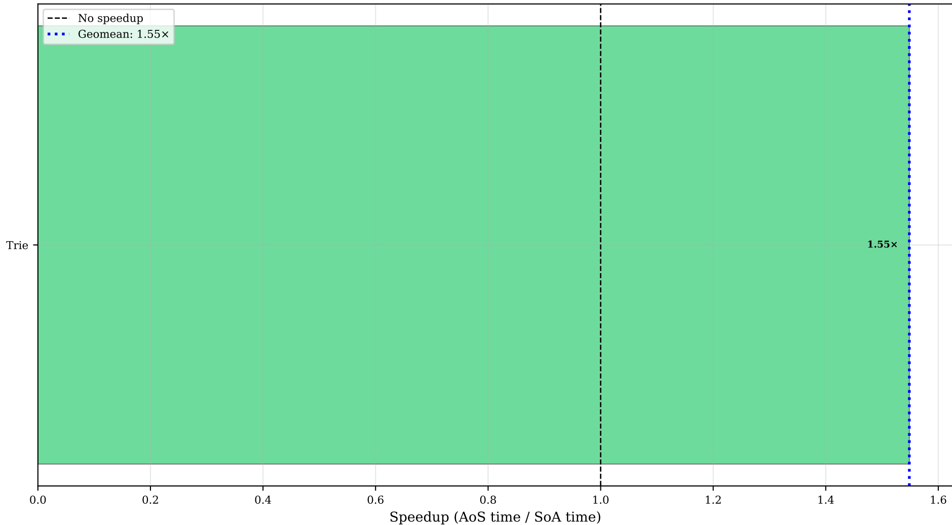
scale frequency (map): Speedup Across All Programs ( >1.0 means SoA is faster)
