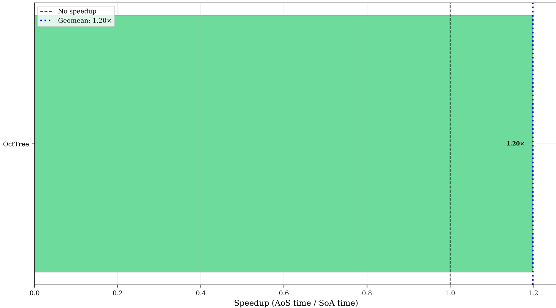
sumEnergy (fold): Speedup Across All Programs (>1.0 means SoA is faster)
