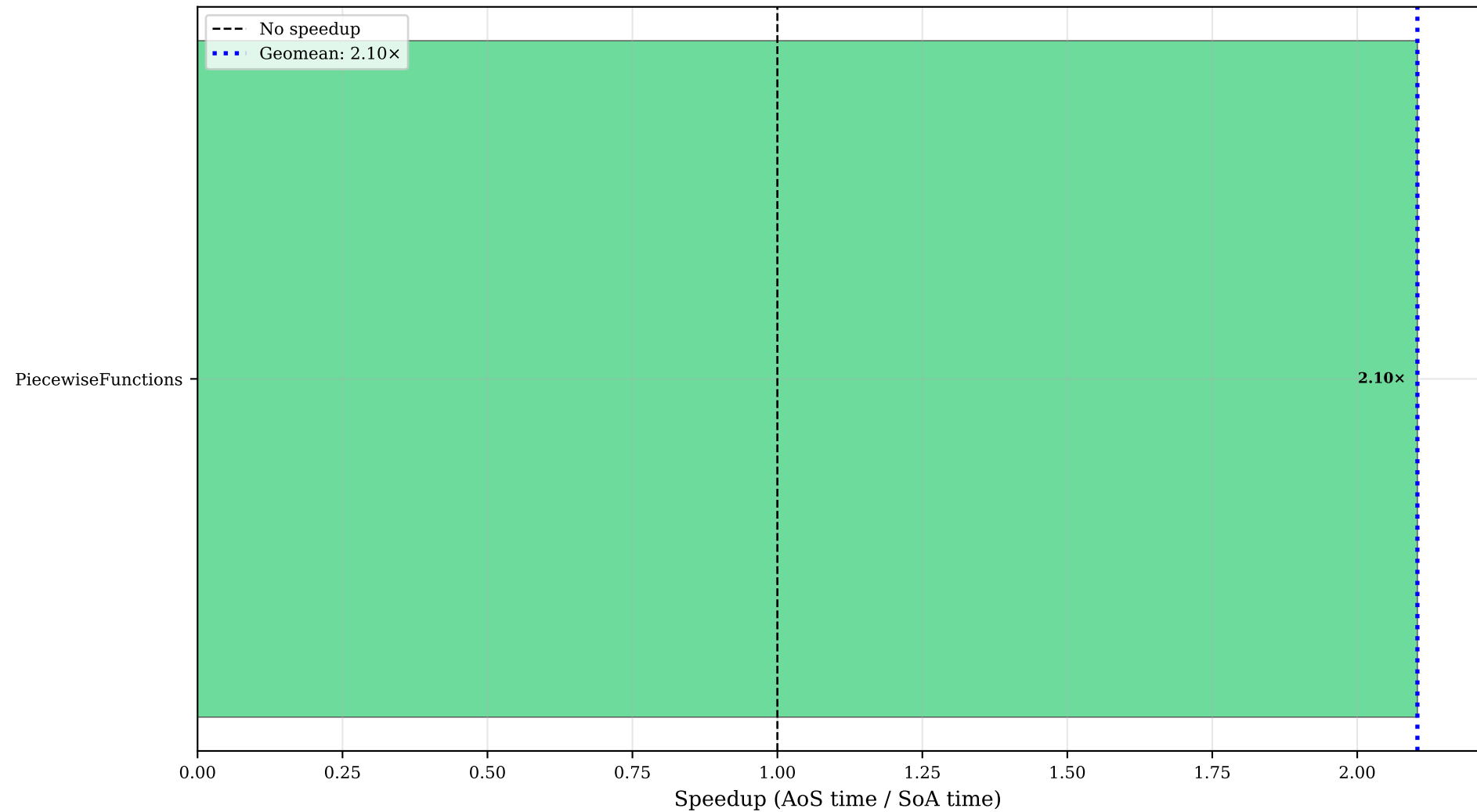
sumError (fold): Speedup Across All Programs (>1.0 means SoA is faster)
