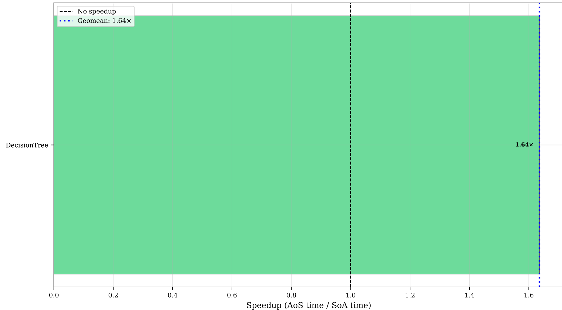
sumImpurity (fold): Speedup Across All Programs (>1.0 means SoA is faster)
