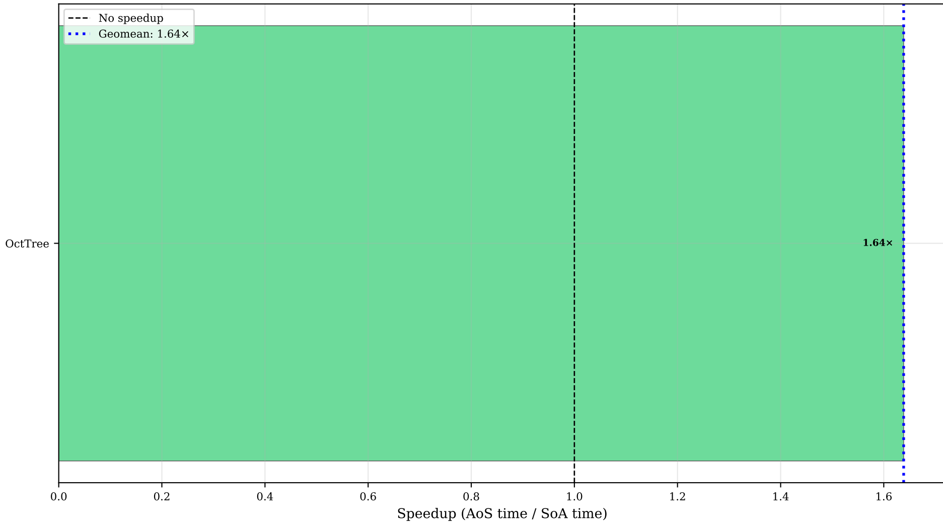
sumMass (fold): Speedup Across All Programs ( >1.0 means SoA is faster)
