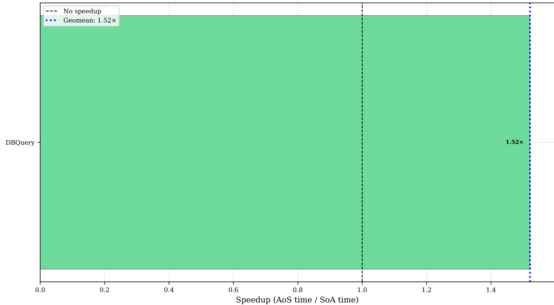
sumMemory (fold): Speedup Across All Programs ( >1.0 means SoA is faster)
